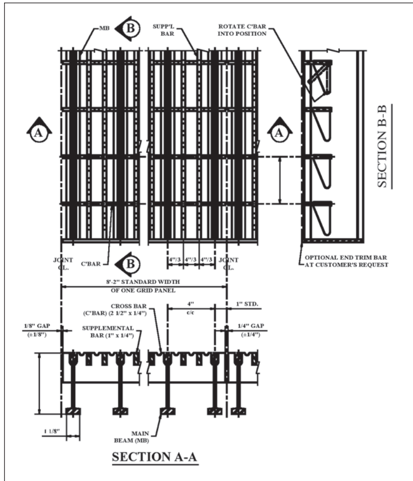
Typical Details: 5-Inch RB 4.2M
