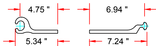
Flange Dimensions
