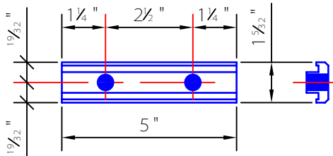
CLAMP BAR
