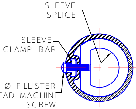
SECTION @ SPLICE
