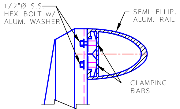
CLAMP BARS
