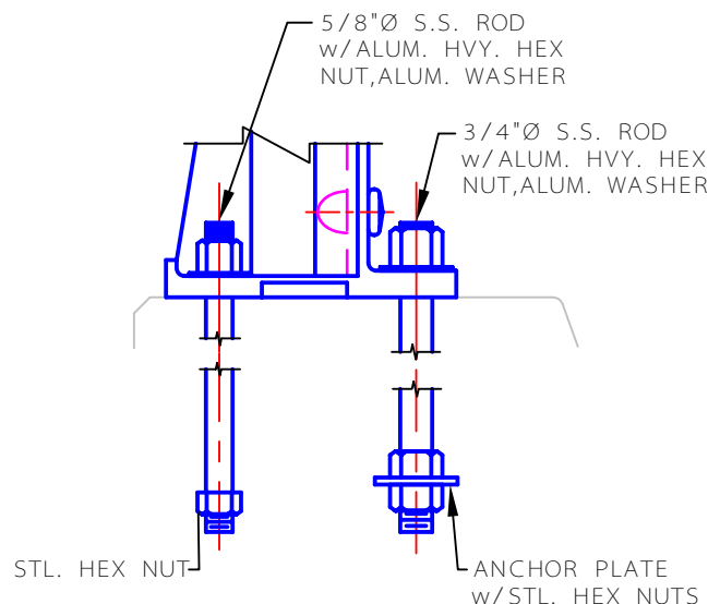
RAIL CAP
