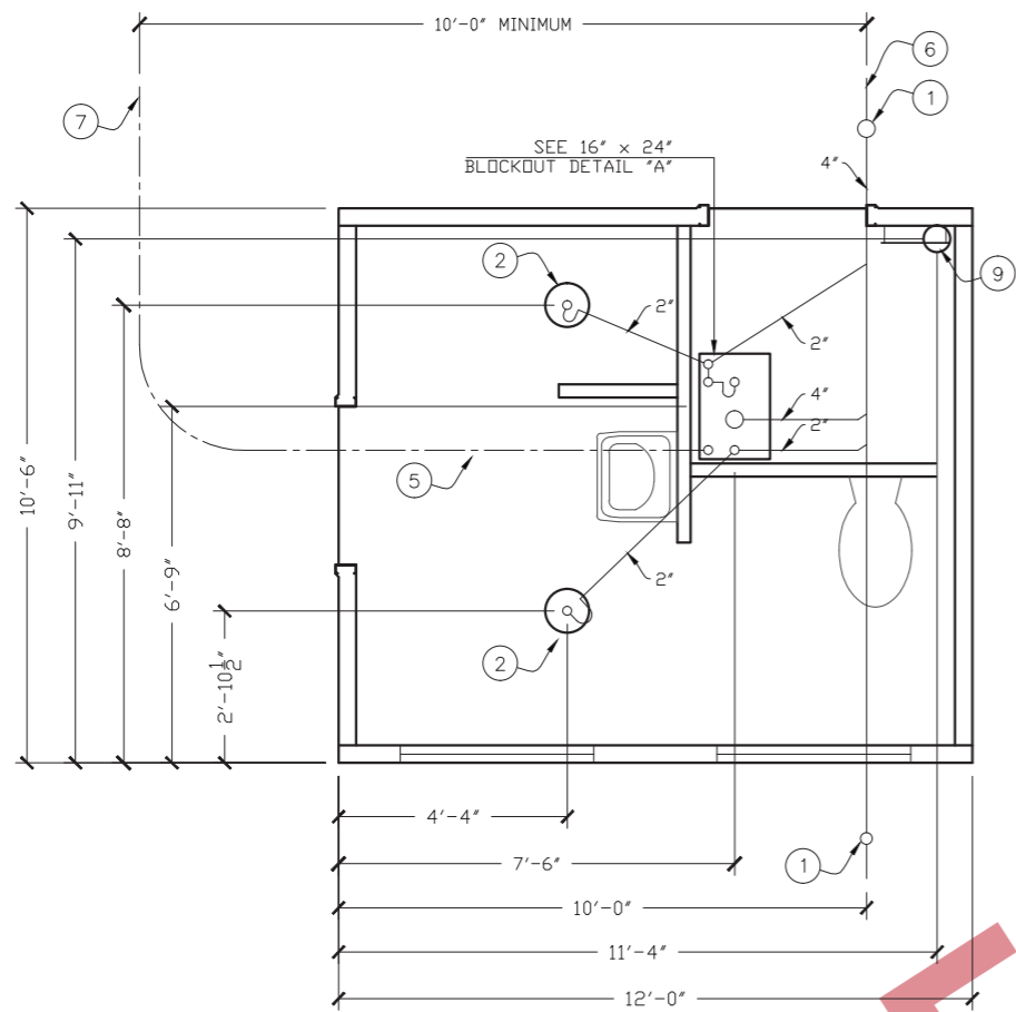
FLOOR DRAIN BLOCKOUTS & BELOW FLOOR PIPING
