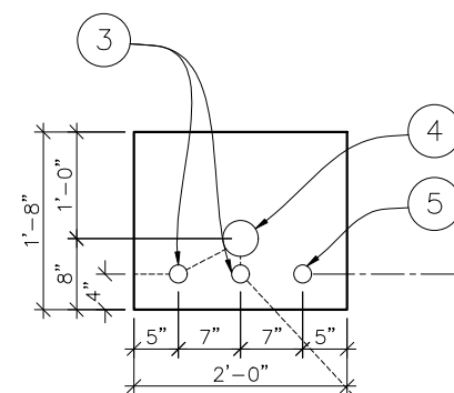
24"x20" BLOCKOUT DETAIL "B"
