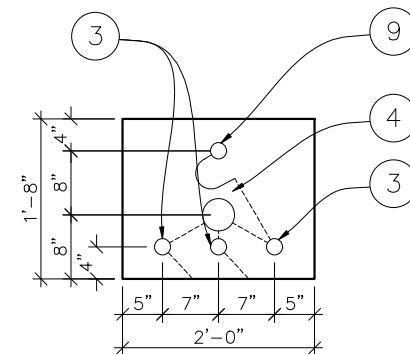
24"x20" BLOCKOUT DETAIL "A"
