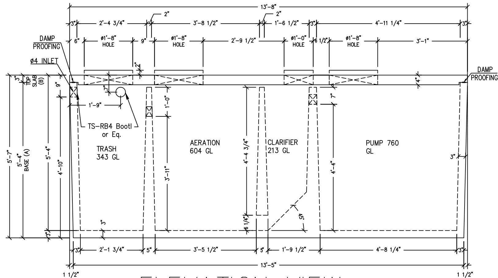
ELEVATION VIEW
