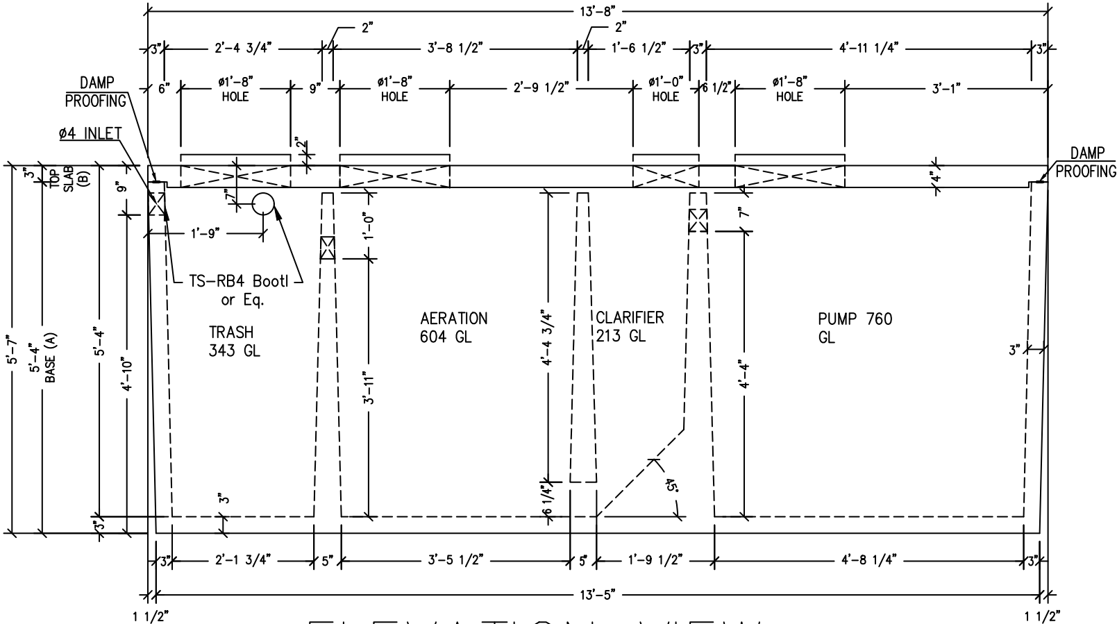
ELEVATION VIEW
