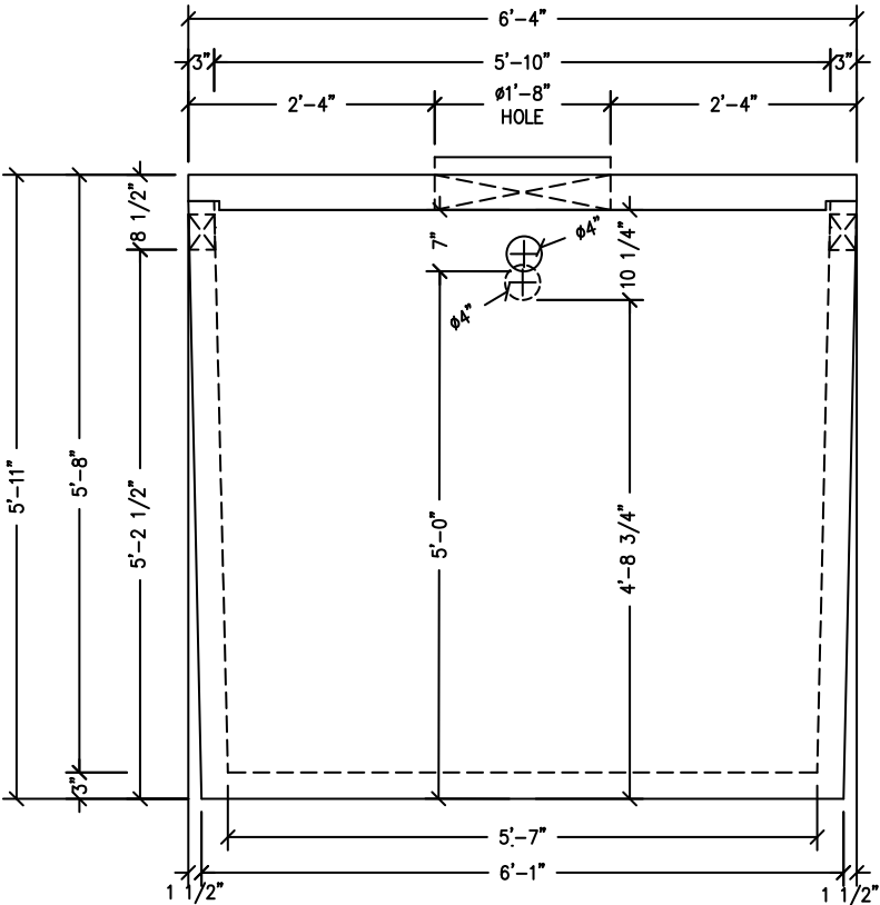
END VIEW
