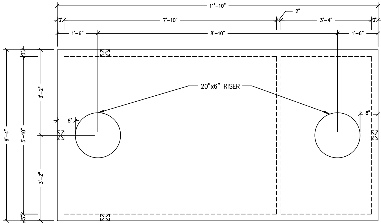
PLAN VIEW
