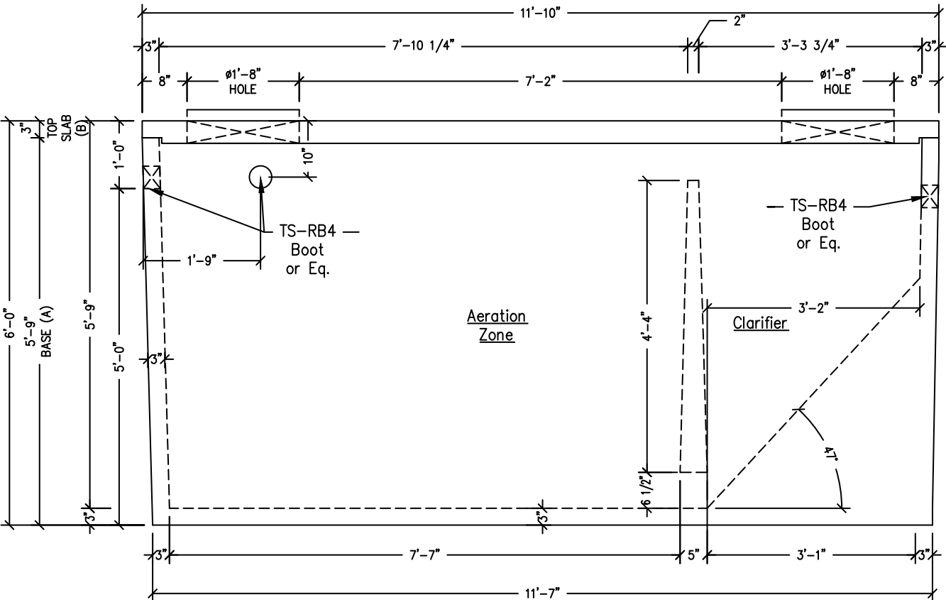
ELEVATION VIEW
